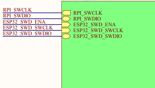
Programming SE0D81B3_5.SchDoc
